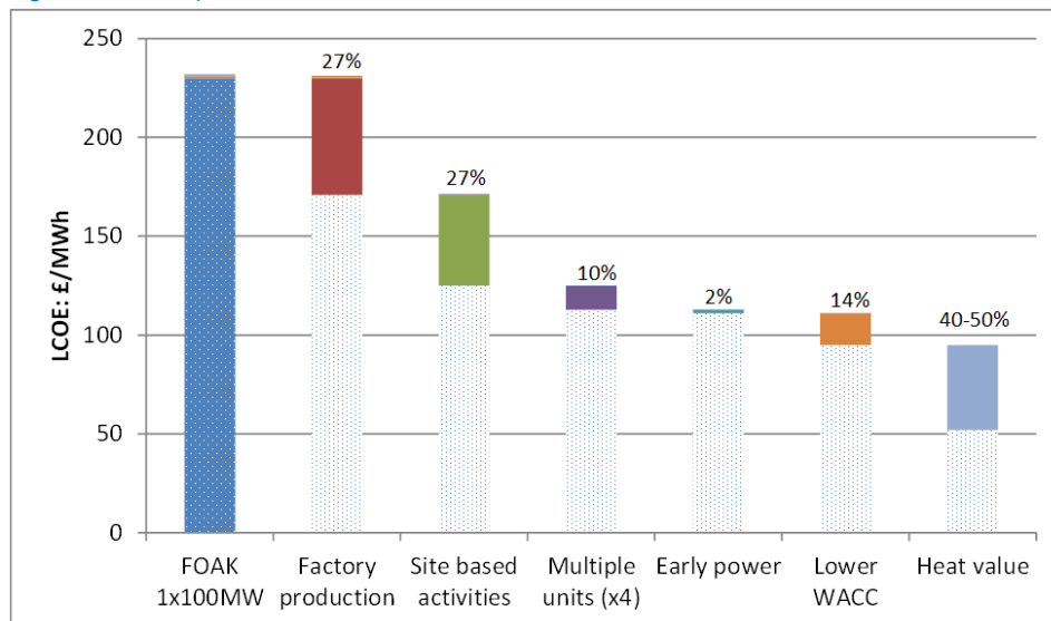
Figure 4.3: Impact of main cost reduction drivers in our SMR cost scenario
